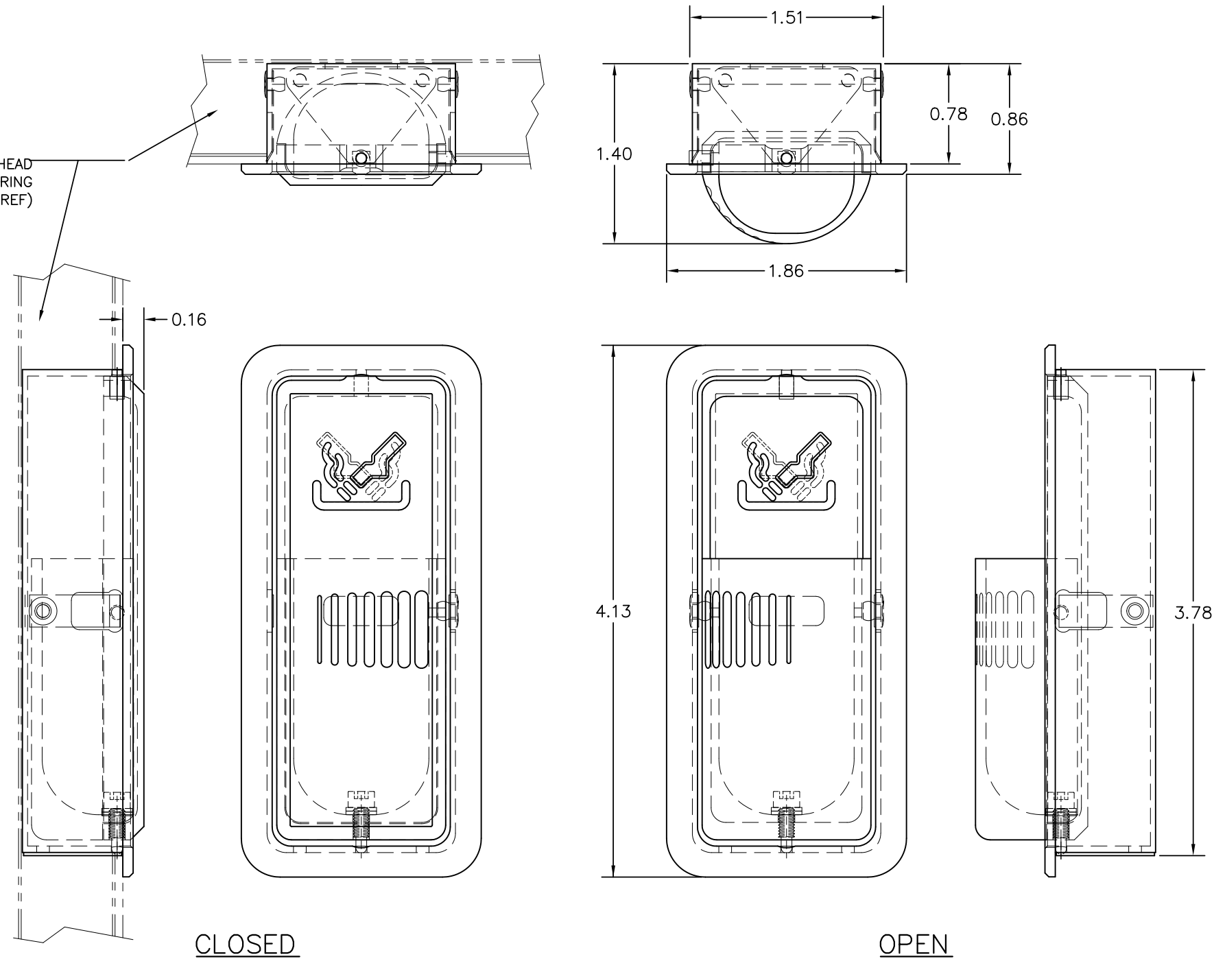
ILLUSTRATION SHOWN WITH A CUSTOMER SUPPLIED ELECTROPLATED FINISH. STANDARD FINISH IS RAW SATIN ALUMINUM READY FOR FINAL POLISHING AND PLATING.
