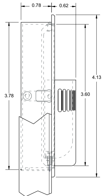
Ashtray shown in open position mounted in 0.50 inch thick vertical panel.*
