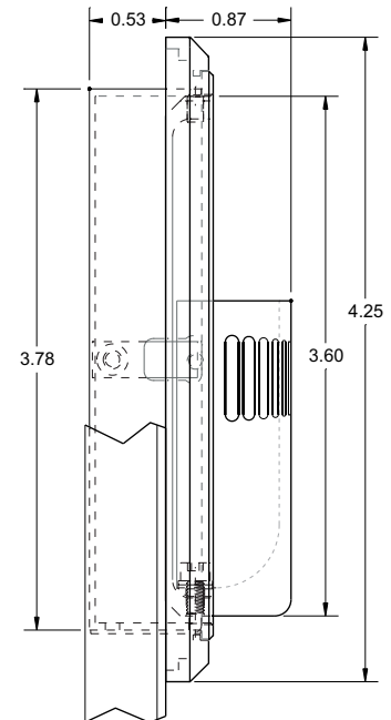
Ashtray shown in open position mounted in 0.50 inch thick vertical panel.*
