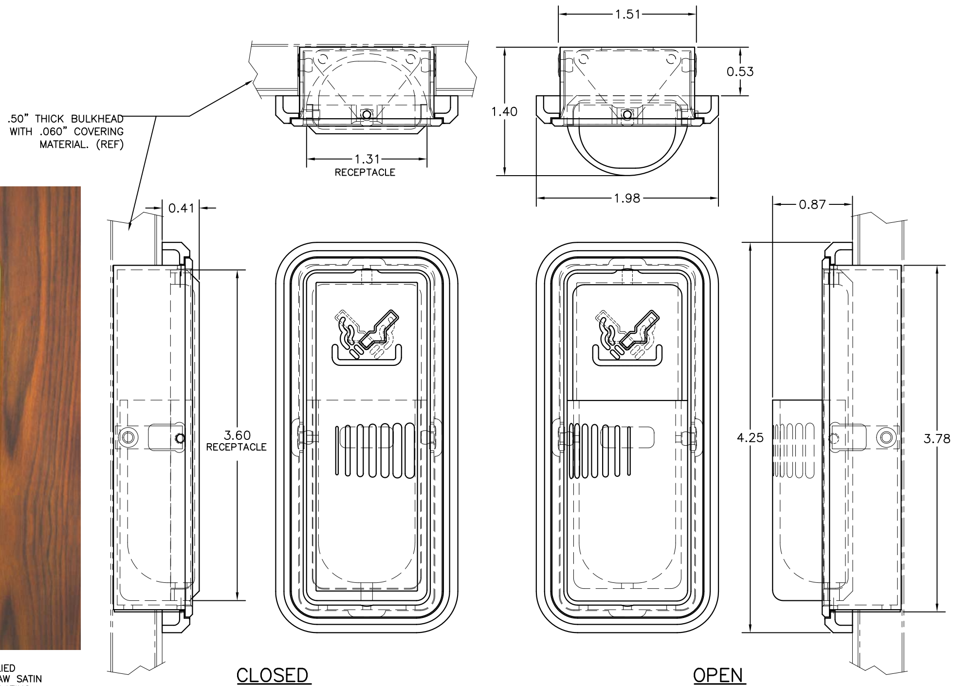
ILLUSTRATION SHOWN WITH A CUSTOMER SUPPLIED ELECTROPLATED FINISH. STANDARD FINISH IS RAW SATIN ALUMINUM READY FOR FINAL POLISHING AND PLATING.
